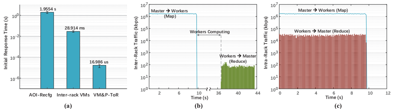
Fig. 2. Experimental results on (a) Initial response time, (b) Inter-rack traffic caused by a WordCount job in traditional O-DCN without in-network computing, and (c) Intra-rack traffic due to running a WordCount job in our P4INC-AOI.
