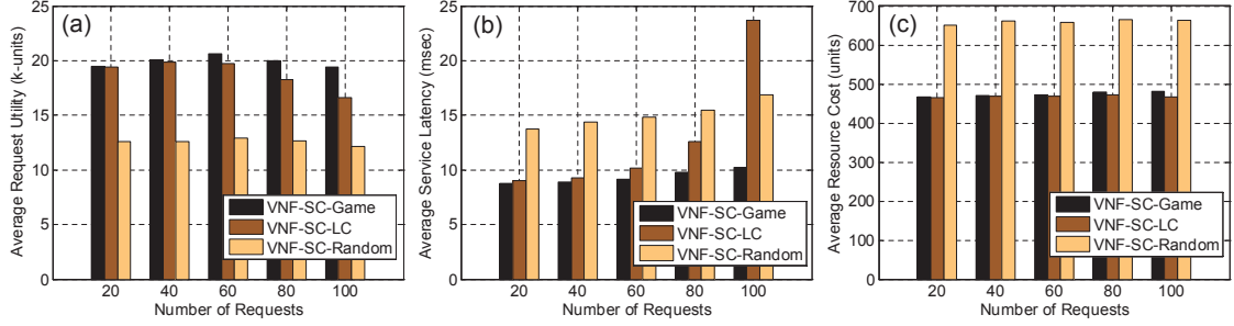
Fig. 6. (a) Request utility, (b) end-to-end service latency and (c) resource consumption cost per request (NSFNET topology, \zeta_{n,m} = 1400 Gb/s).
