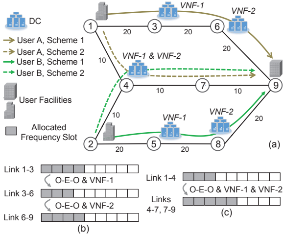
Fig. 1. Example for incentive-driven VNF-SC provisioning in IDC-EONs: (a) case description, (b) and (c) spectrum allocation for paths 1-3-6-9 and 1-4-7-9 respectively.
